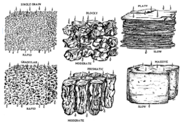
Figure 3: Classification of soil aggregates and their average water flow properties (Ref. 4)
