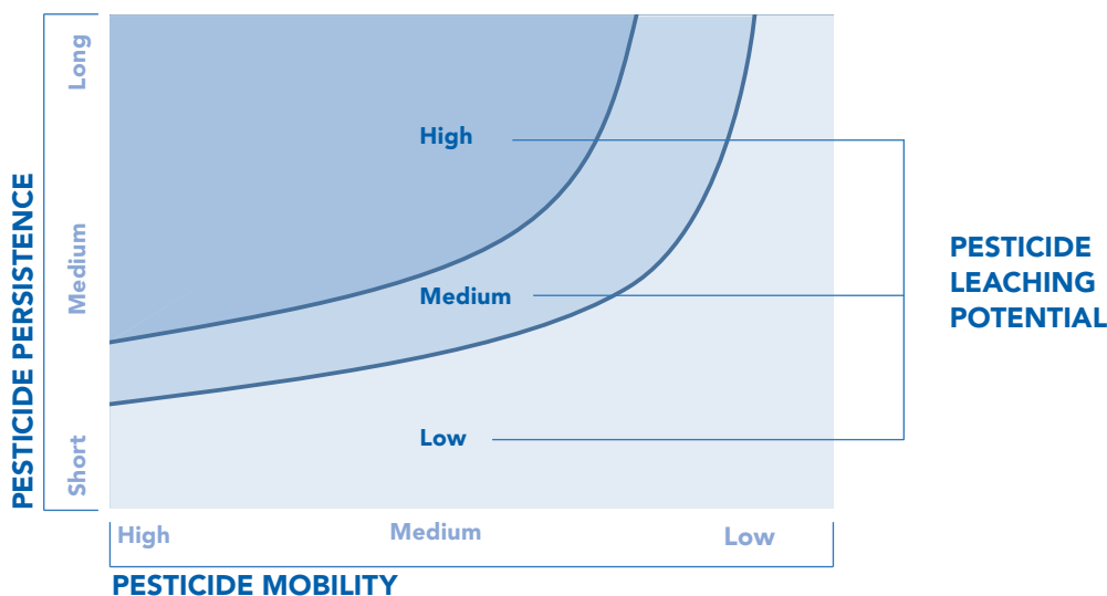
Figure 6: The link between pesticide leaching potential in soil and the persistence and mobility of pesticides in soil (based on the GUS concept)
