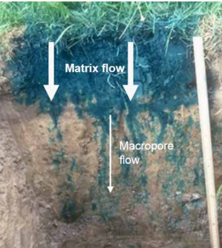
Figure 7: Water flow pattern in a soil profile (left side) and staining pattern of macropores (right side) made visible via infiltration experiments with colour tracer (Ref. 9)
