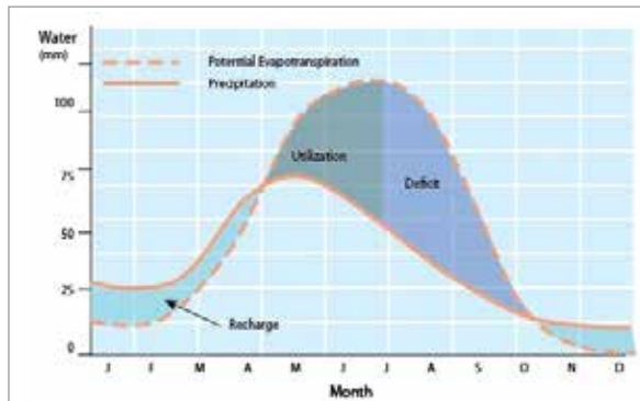
Figure 5: Seasonal soil-water balance example (Ref. 8)
