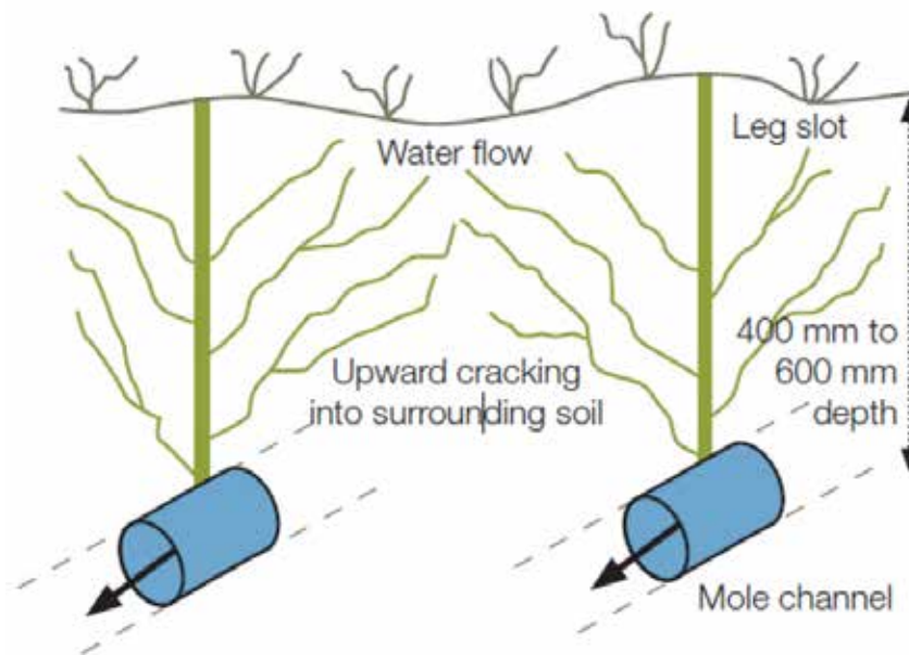
Figure 12: Schematic view of effect of mole drainage in soils (Ref. 14)
