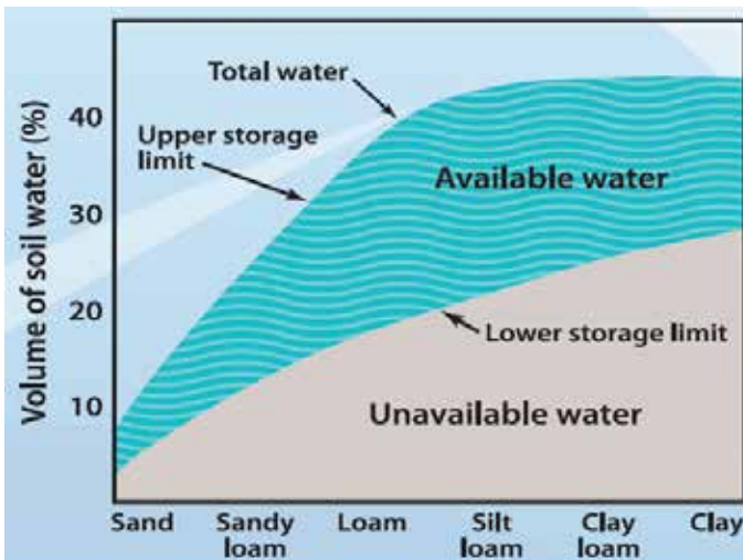
Figure 4: Water storage and plant-water availability depend largely on soil texture (Ref. 6)
