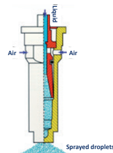
Fig. 11: Air induction nozzles.
