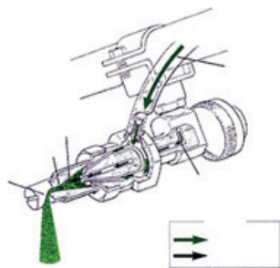
Fig. 27: Twin fluid nozzle.
