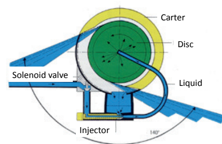
Fig. 22: Rotary atomizers.
